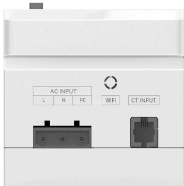
NeuronIII(N3)-Lite Top-view
