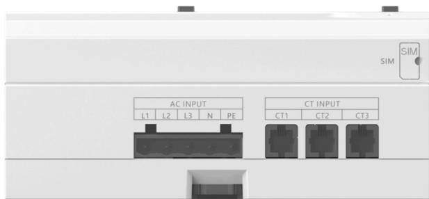
NeuronIII(N3) Top-view
