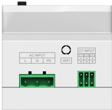
NeuronIII(N3)-Lite-3P Top-view
